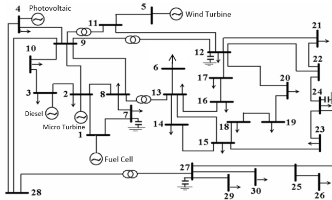
Fig. 2. Modified IEEE thirty-bus test [9].
